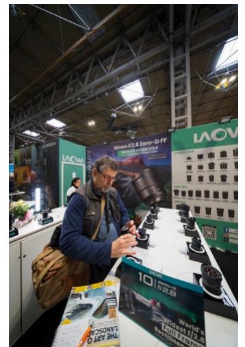
Checking geometry on both horizontal (above) and vertical (right) frames matters as distortion may vary with distance from the axis.
