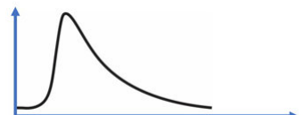
Typical flash output at full setting (left) and 1/16 th (right). The timing at the fastest focal plane shutter sync speed is just before the rise in output so always gets most of the duration – but precise timing adjustment in microseconds is needed for very fast global shutter speeds to match the peak output.
